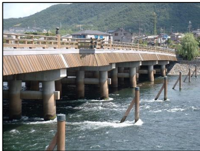
Uji-bashi Bridge
